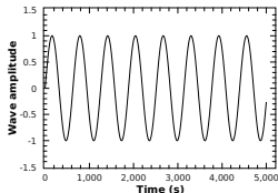
Sound wave at single frequency.
