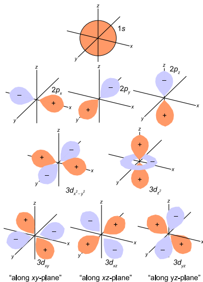
Plots demonstrating the shapes of different hydrogenlike atomic orbitals.
