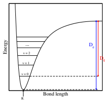
Definitions of D_e and D_0 .
