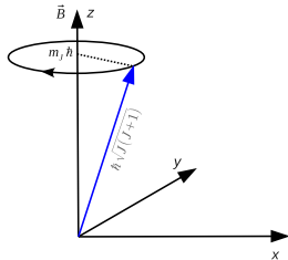
Single spin Larmor precession about z
