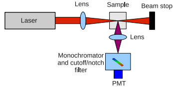
Typical Raman experiment setup.
