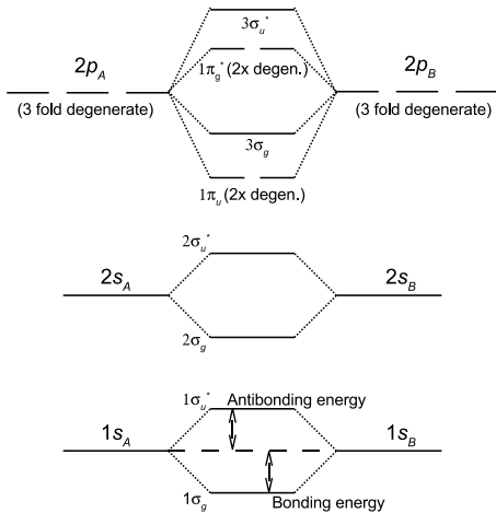
MO diagram for homonuclear diatomic molecules.
