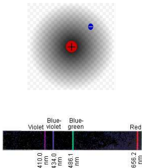
Emission spectrum of hydrogen atom
