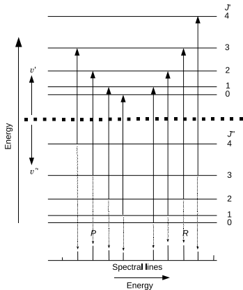
Both v and J change in transitions.
