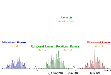
Example of rotation-vibration Raman spectrum ( N_2 gas)
