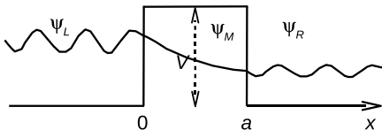
Wavefunction for a particle with E < V tunneling through a potential barrier
