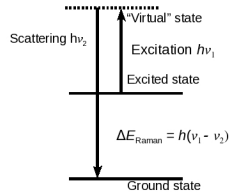
Raman process (anti-Stokes)
