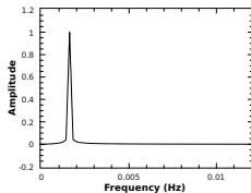
Power spectrum of the sound wave.
