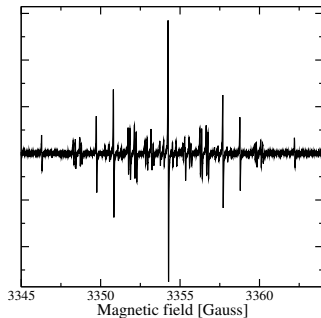
EPR spectrum of hydroquinone cation radical
