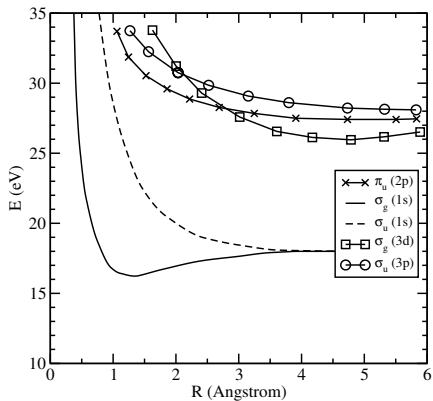
The lowest excited states of \text{H}_2^+ .
