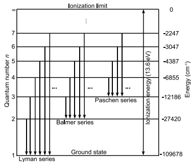
H atom emission lines
