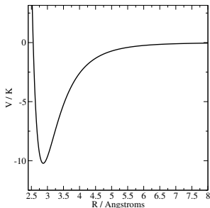
Pair potential between two helium atoms.
