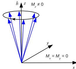
An ensemble of spins precessing about z
