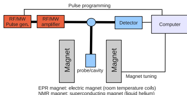
NMR/EPR block diagram (pulsed instrument).
