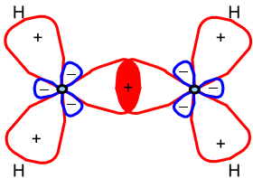
Formation of \sigma bonds from hybrid orbitals.
