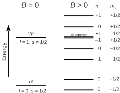
Splitting of hydrogenlike atom energy levels in external magnetic field
