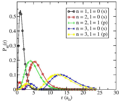
Radial probabilities P_{nl}(r) .
