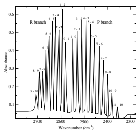
Vibration-rotation spectrum of HBr molecule in the gas phase. The peaks are labeled according to their initial (first) and final (last) rotational states.
