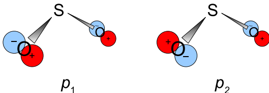
p_1 and p_2 basis functions in \text{SO}_2 .
