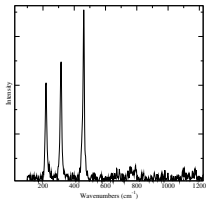
Example of vibration Raman spectrum ( CCl_4 liquid)
