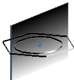
One of the \sigma_v planes going through the center and the two carbons
