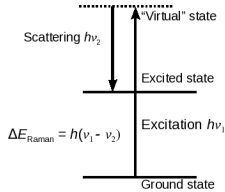
Raman process (Stokes)
