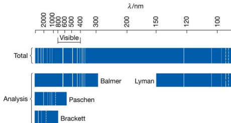
Emission spectrum of atomic hydrogen.
