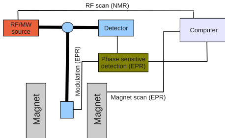
NMR/EPR block diagram (CW).
