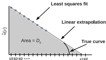
Example of Birge-Sponer plot.
