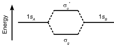
MO diagram showing the \sigma_g and \sigma_u molecular orbitals.
