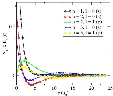
Radial wavefunctions N_{nl} \times R_{nl}(r) .
